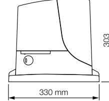
RB600/RB1000
